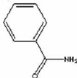
Fig.1. Molecular structure of benzamide
